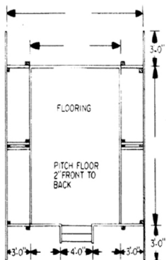
FLOOR PLAN
