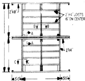
FRAMING AND FOUNDATION
