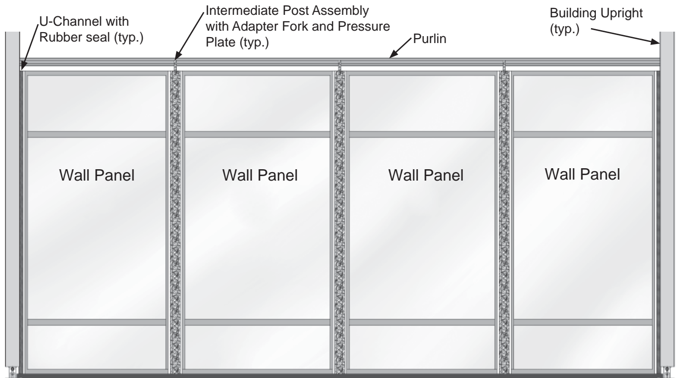
ELEVATION Outside View
