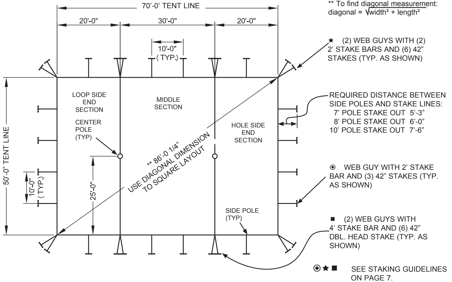
Staking Table For Single Pole
